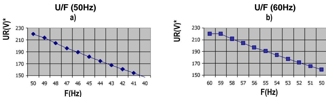
Figure 12.1: Actuation point for U/F protection
