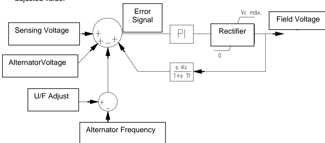
Figure 5.2: Control diagram of AVR-A-OPT-03
