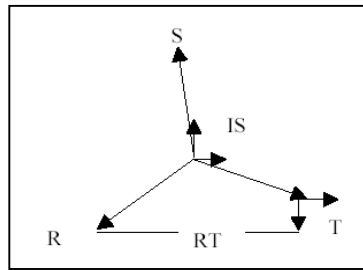
Figura 11.1: Diagrama fasorial
