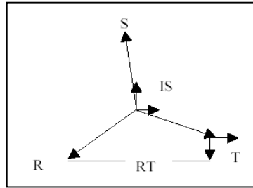
Figura 11.1: Diagrama fasorial
