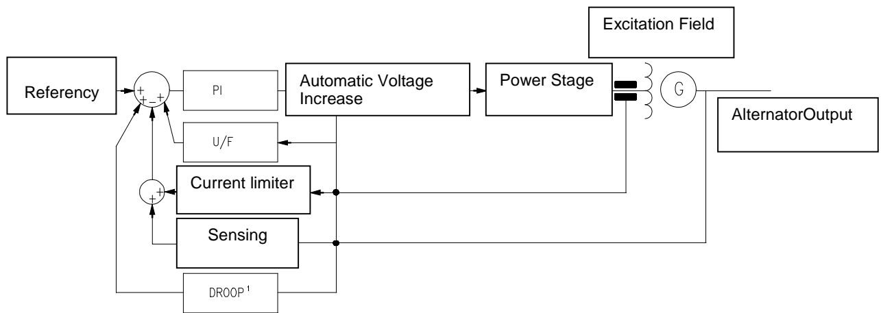
Figure 5.1: Voltage regulator block diagram
